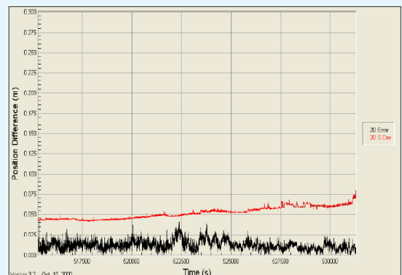
Figure 5: SMART-V1G Typical RT-20 Steady State (Horizontal)
