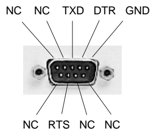
Figure 22 Pinout for TIME Port - GUS
