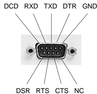
Figure 8 Pinout for L1-C/A, L1/L2 I, & L1/L2 II Ports - WAAS
