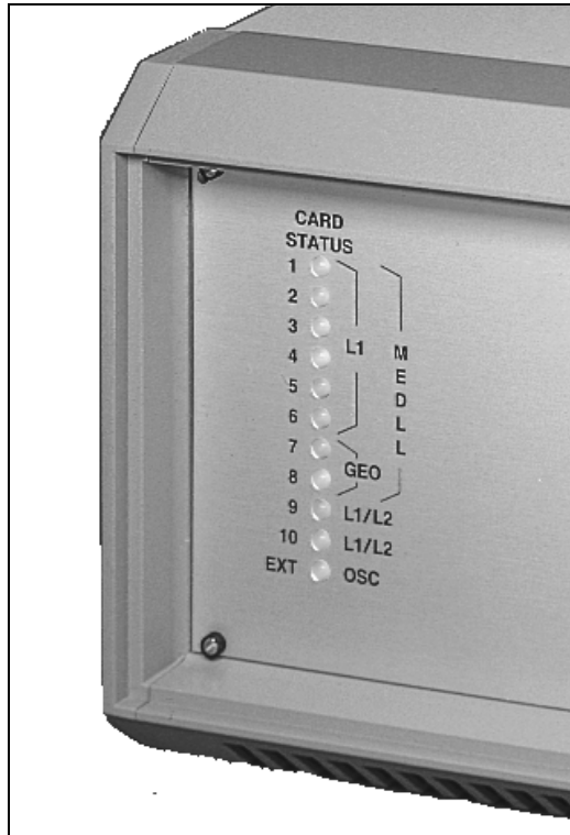
Figure 20 Lights on Front Panel of GUS Receiver
