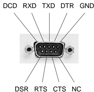
Figure 21 Pinout for L1-C/A, L1/L2 I, & L1/L2 II Ports - GUS
