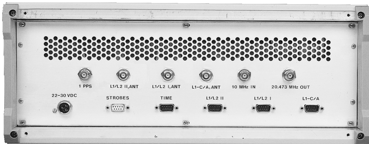
Figure 18 Rear Panel of GUS Receiver
