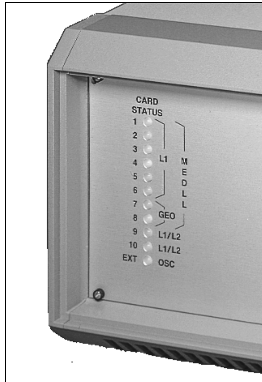
Figure 7 Lights on Front Panel of WAAS Receiver
