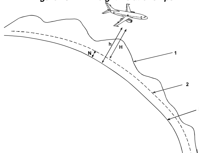
Figure 16 Height Relationships
