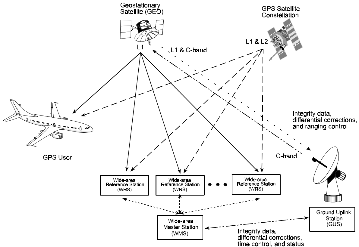
Figure 1 The WAAS Concept
