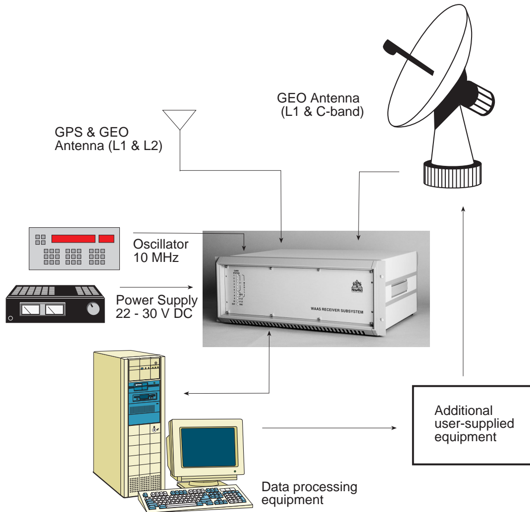
Figure 17 GUS Minimum System Configuration
