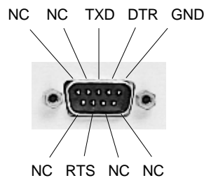
Figure 9 Pinout for TIME Port - WAAS
