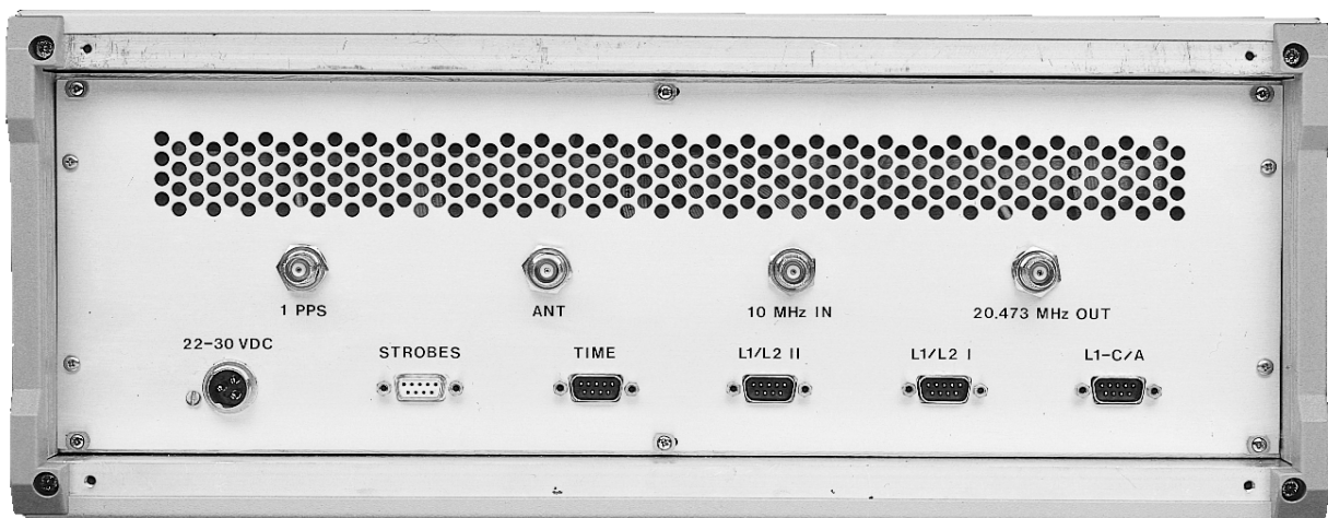
Figure 5 Rear Panel of WAAS Receiver
