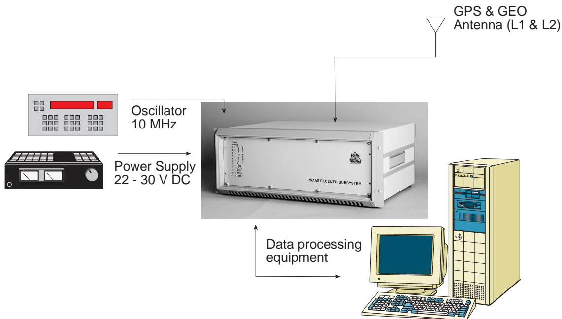
Figure 4 WAAS Minimum System Configuration
